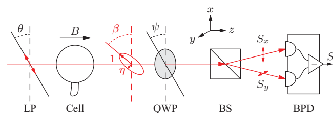
FIG. 2. (Color online) Experimental setup for the GLL. LP: Linearly polarized light, B : Applied magnetic field, QWP: Quarter-wave plate, BS: Beam splitter (Wollaston prism), BPD: Balanced photodetector. \theta is set by the input half-wave plate angle, and \psi is the QWP angle.
