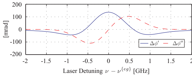
FIG. 1. (Color online) Real and imaginary parts of the gyrotropic angle \Delta\phi for a length \ell = 1.86 cm of saturated potassium vapor (93.3% ^{39}\text{K} and 6.7% ^{41}\text{K} ) at temperature T = 60^\circ\text{C} , a magnetic field B = 150 G, and a laser frequency \nu close to the zero-field mean frequency \nu^{(eg)} of the 770.1 nm line of ^{39}\text{K} .
